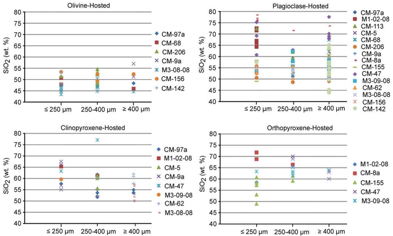
Fig. 11. Melt inclusion SiO 2 compositions by host phenocryst size. Host phenocryst sizes are split into categories small (1; ≤250 μm), medium (2; 250–400 μm), and large (3; ≥400 μm).
