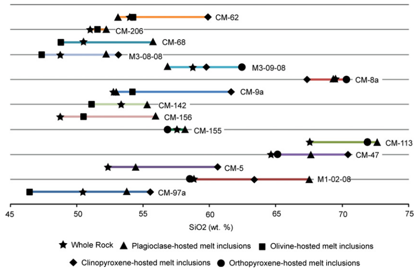
Fig. 8. Average SiO 2 values for melt inclusions in every host mineral, compared with whole-rock values, for every sample. Each line represents the range in average values for a given sample. Standard deviations for SiO 2 values in melt inclusions from each host mineral are as follows: plagioclase: average 1.03, range 0.21–3.65 wt.%; olivine: SiO 2 : average 1.02, range 0.32–3.24 wt.%; cpx: average 1.49, range 0.40–4.10 wt.%; opx: 1.78, range 0.63–4.55 wt.%. Samples where the whole-rock composition is less evolved than all the average melt inclusion data provide unambiguous evidence for addition of a basaltic magma just before eruption. Hence, magma mixing appears likely to trigger volcanic eruptions.
