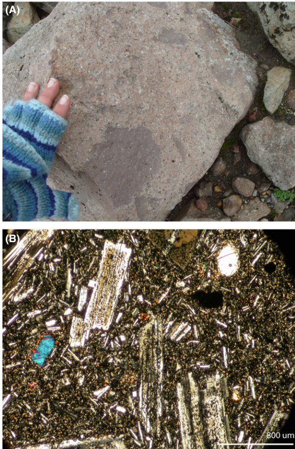
Fig. 10. Visual evidence consistent with magma mixing observed in the field (A) and in thin section (B). Part (A) shows mafic enclaves with chilled margins hosted in a more felsic matrix. Part (B) shows abundant sieve-textured plagioclase.
