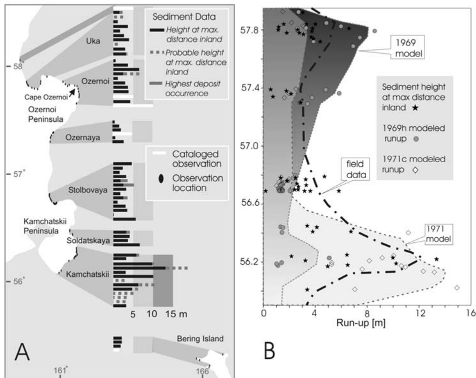
Figure 2. (a) Elevation distribution of tsunami deposits discussed in the text, and heights from catalog [Zayakin and Luchina, 1987] (see also Figures S1, S2, and S3). “Height at maximum distance inland” is what is usually termed runup, and modeling gives a comparable value, at the limit of inundation. Maximum height of the deposit, where that number is greater than runup, is also given. (b) Comparison of field sediment heights to runup modeled for the 1969 and 1971 tsunamis, plotted by latitude. Dot-dash line shows envelope of field sediment runup, excepting outliers. Shaded areas, shown for visual ease, are very simplified because runup models were run only where we had topographic profiles; see Figure 3 for the overall pattern of tsunami amplitude. Modeled runup should exceed sediment runup (field data) to satisfy conditions for a fit. The 1969 model exceeds field data in the north, the 1971 model exceeds field data in the south, and neither exceeds the data in the middle.
