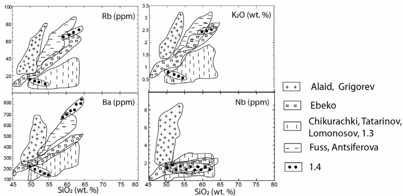
Figure 2. Harker's diagrams. Variations of major and trace elements in the volcanic rocks from the Northern Kuril Islands.
